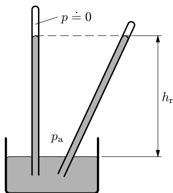
Obr. 15 Torricelliho pokus
