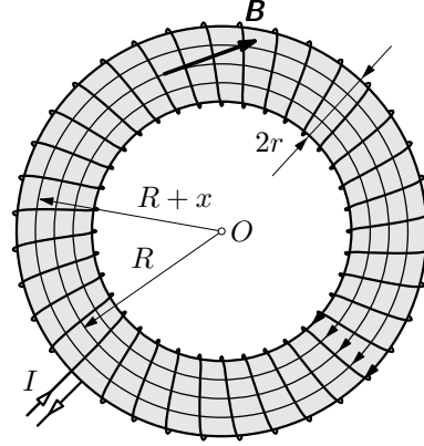
Obr. 19 Toroid
